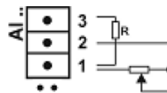
- Resistance transmitter
